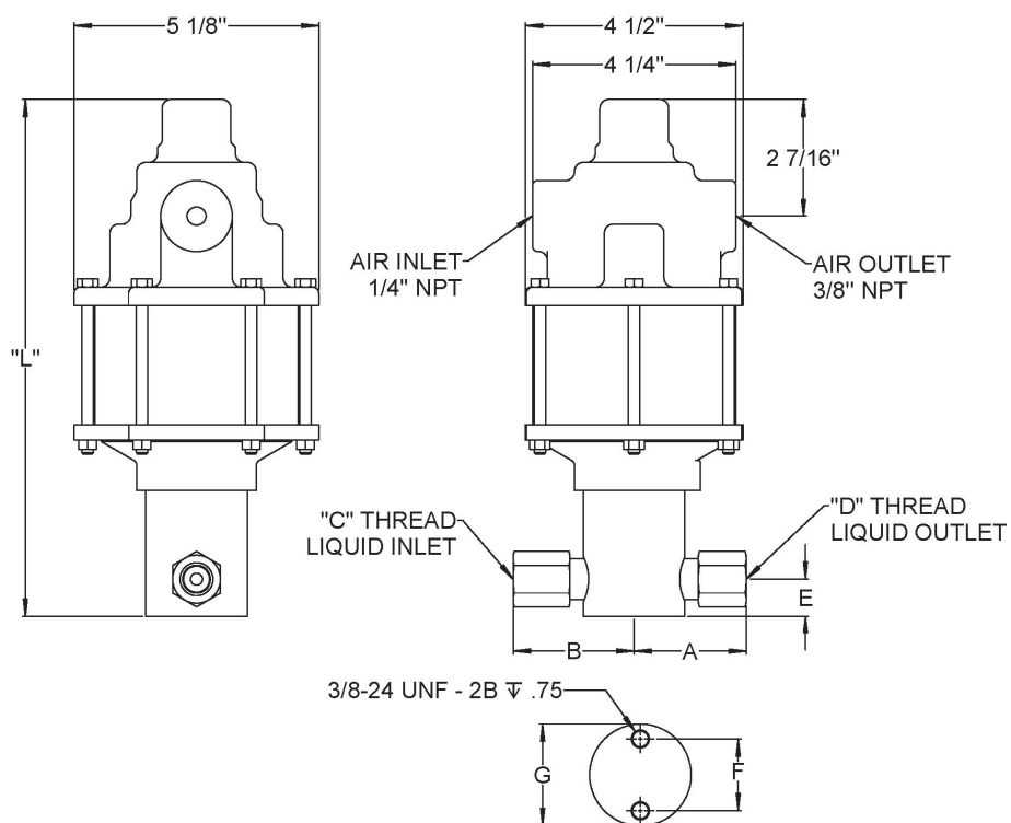
Mounting Dimensions in Inches
