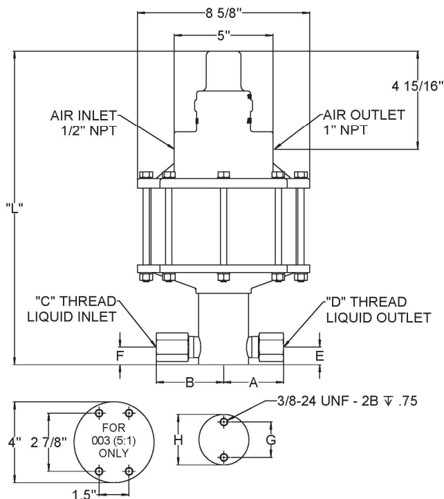
Mounting Dimensions in Inches
